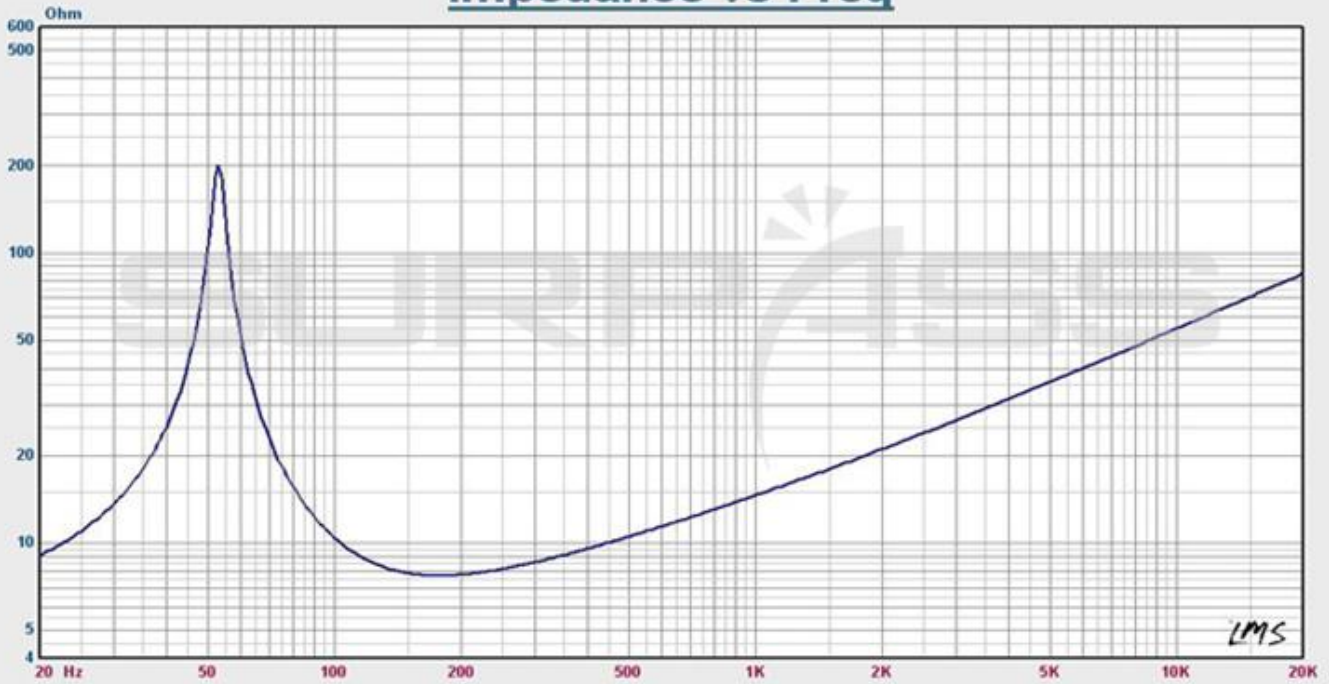
Impedance vs Freq
